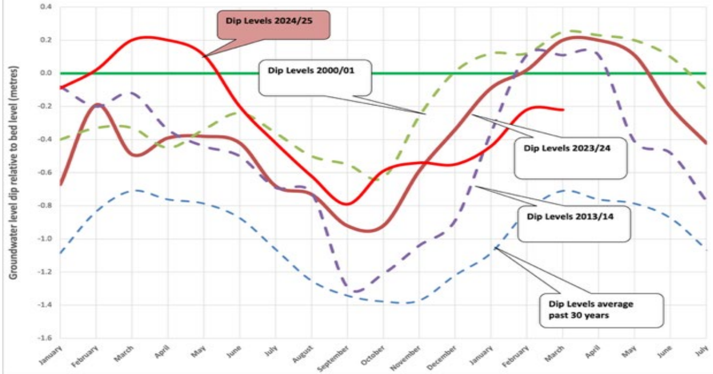
18 MONTH AMERSHAM CHURCH GROUNDWATER LEVELS VS BED LEVEL
